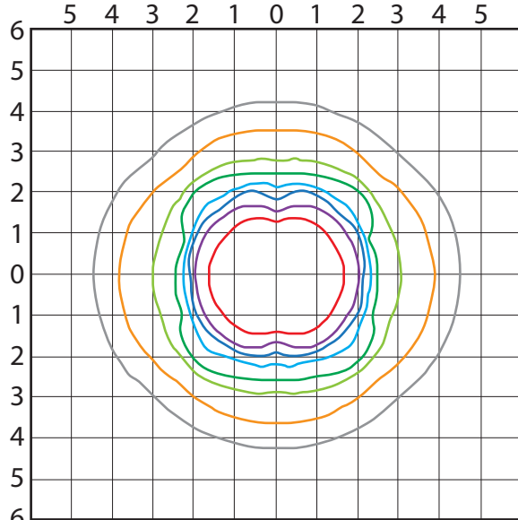
906602 AC/DE Fusion 8 in Air-Cooled Iso Footcandle Plot
