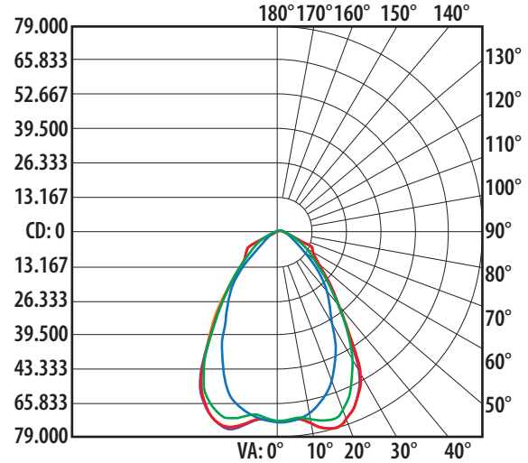
906602 AC/DE Fusion 8 in Air-Cooled Polar Candela Distribution
