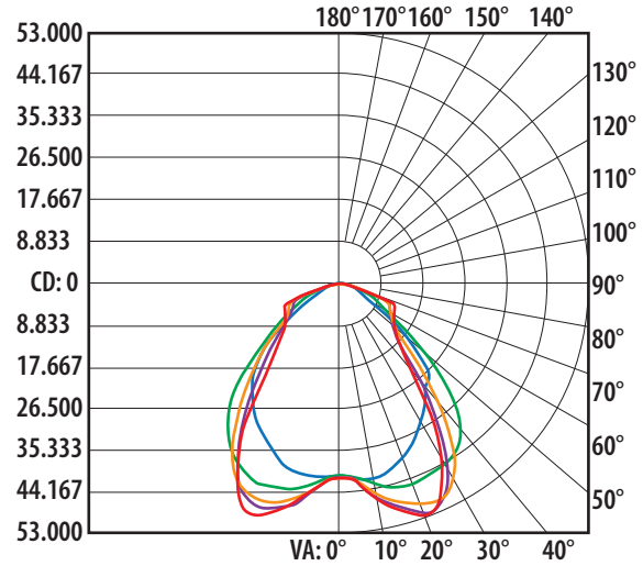
904938 Flex DE Polar Candela Distribution
