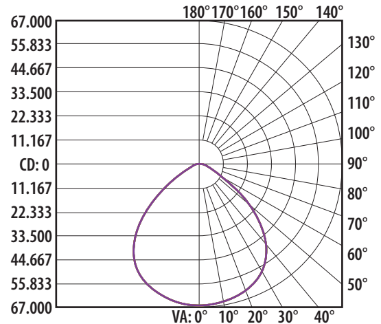
904916 Silver Sun Polar Candela Distribution
