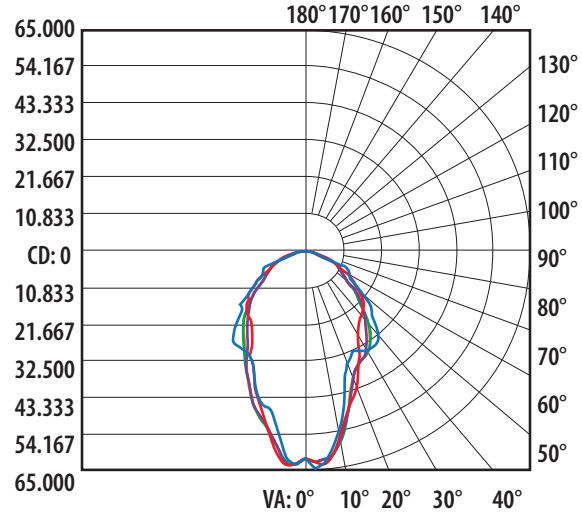
904655 BlockBuster 8 in Air-Cooled Polar Candela Distribution
