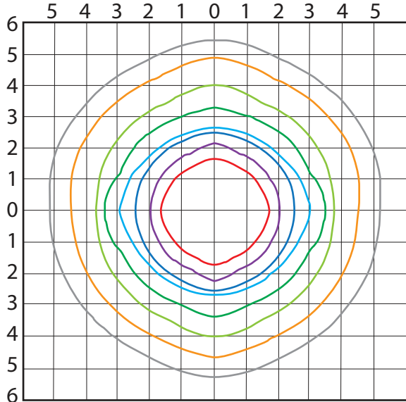
904655 BlockBuster 8 in Air-Cooled Iso Footcandle Plot
