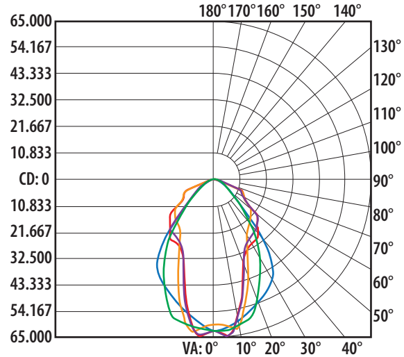
904650 BlockBuster 6 in Air-Cooled Polar Candela Distribution
