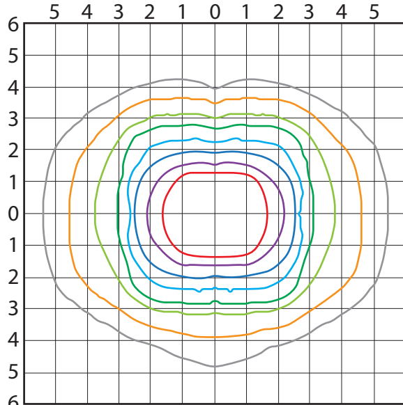
904650 BlockBuster 6 in Air-Cooled Iso Footcandle Plot
