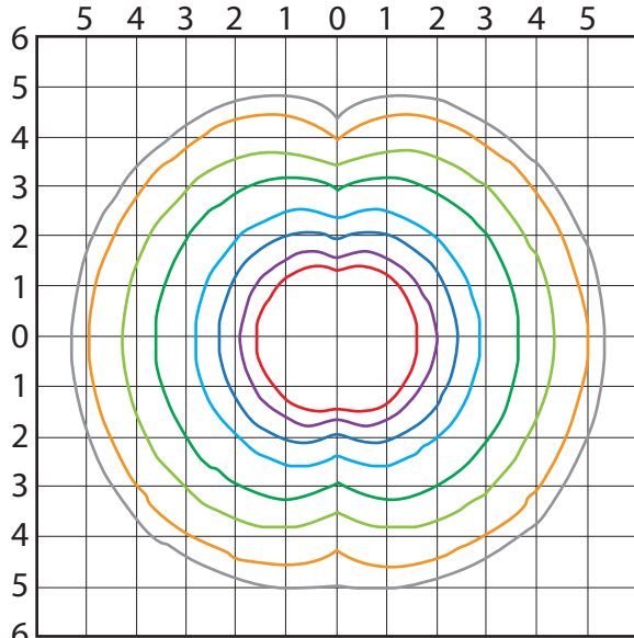
904520 Magnum XXXL 6 in Air-Cooled Iso Footcandle Plot
