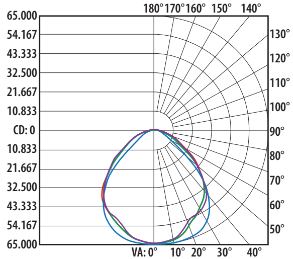
904520 Magnum XXXL 6 in Air-Cooled Polar Candela Distribution
