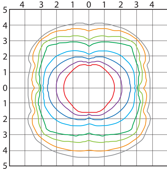
904515 Magnum XXXL 8 in Air-Cooled Iso Footcandle Plot
