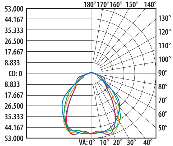
904515 Magnum XXXL 8 in Air-Cooled Polar Candela Distribution
